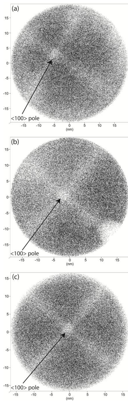
Figure 4. The first 10 nm of the NSC15 (a), HAR5 (b), and microtip (c) reconstructions looking down the analysis direction, all dimensions in nm. The Si <100> pole is highlighted.
