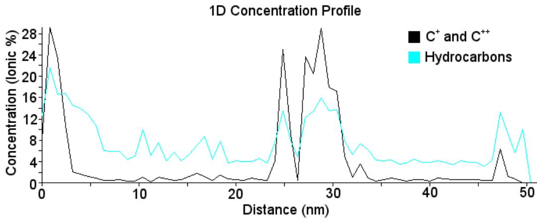
Figure 4. 1D concentration profile showing atomic C and hydrocarbons have a higher concentration at regular intervals through the DLC coating. The profile was taken from a 5 \times 5 \times 50 \text{ nm} region down the center of the tip axis.
