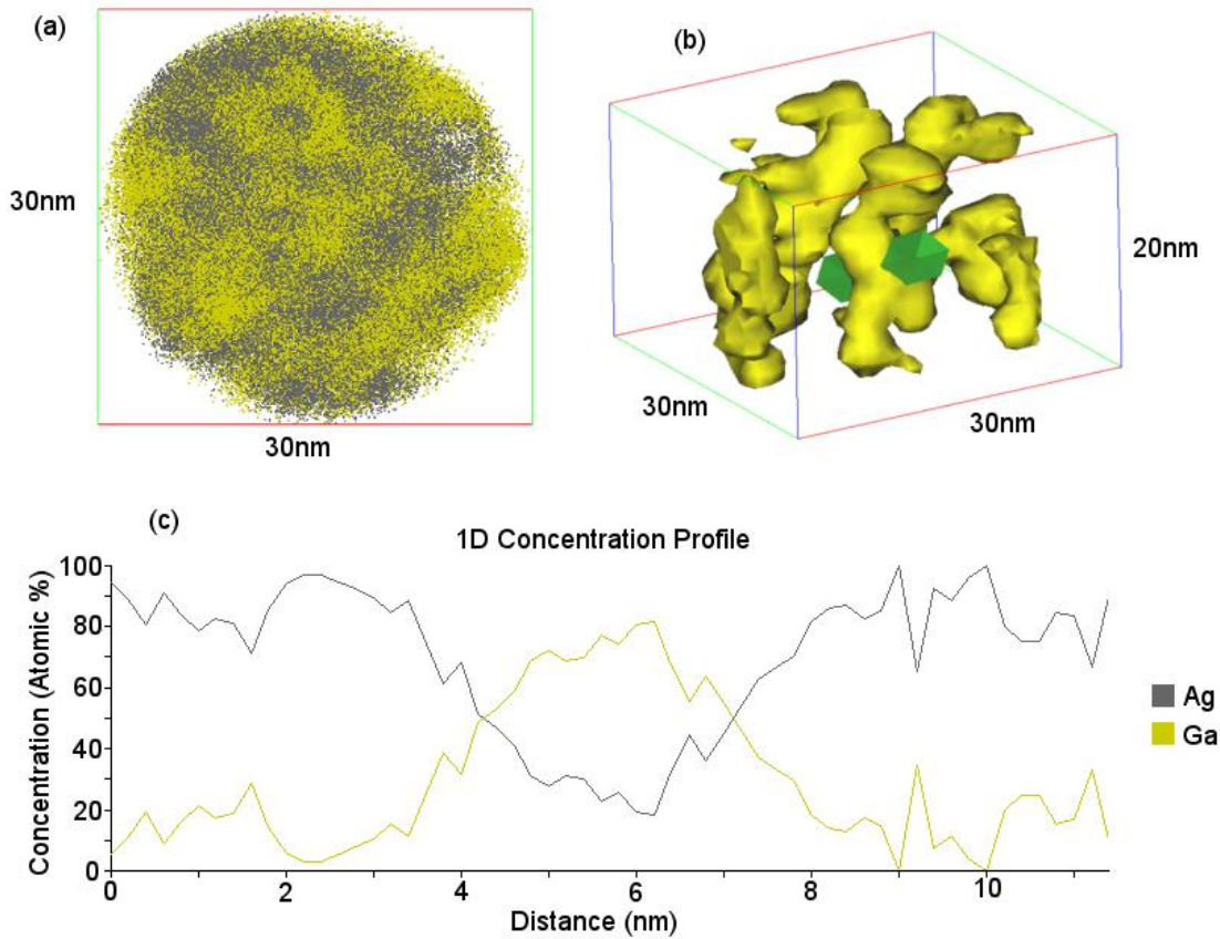
Figure 6. Top view of a NaugaNeedle™ APT reconstruction (a) along with isoconcentration surfaces highlighting the Ga rich zones (b), and a 1D concentration profile (c) along the long axis of the region shown in (b).
